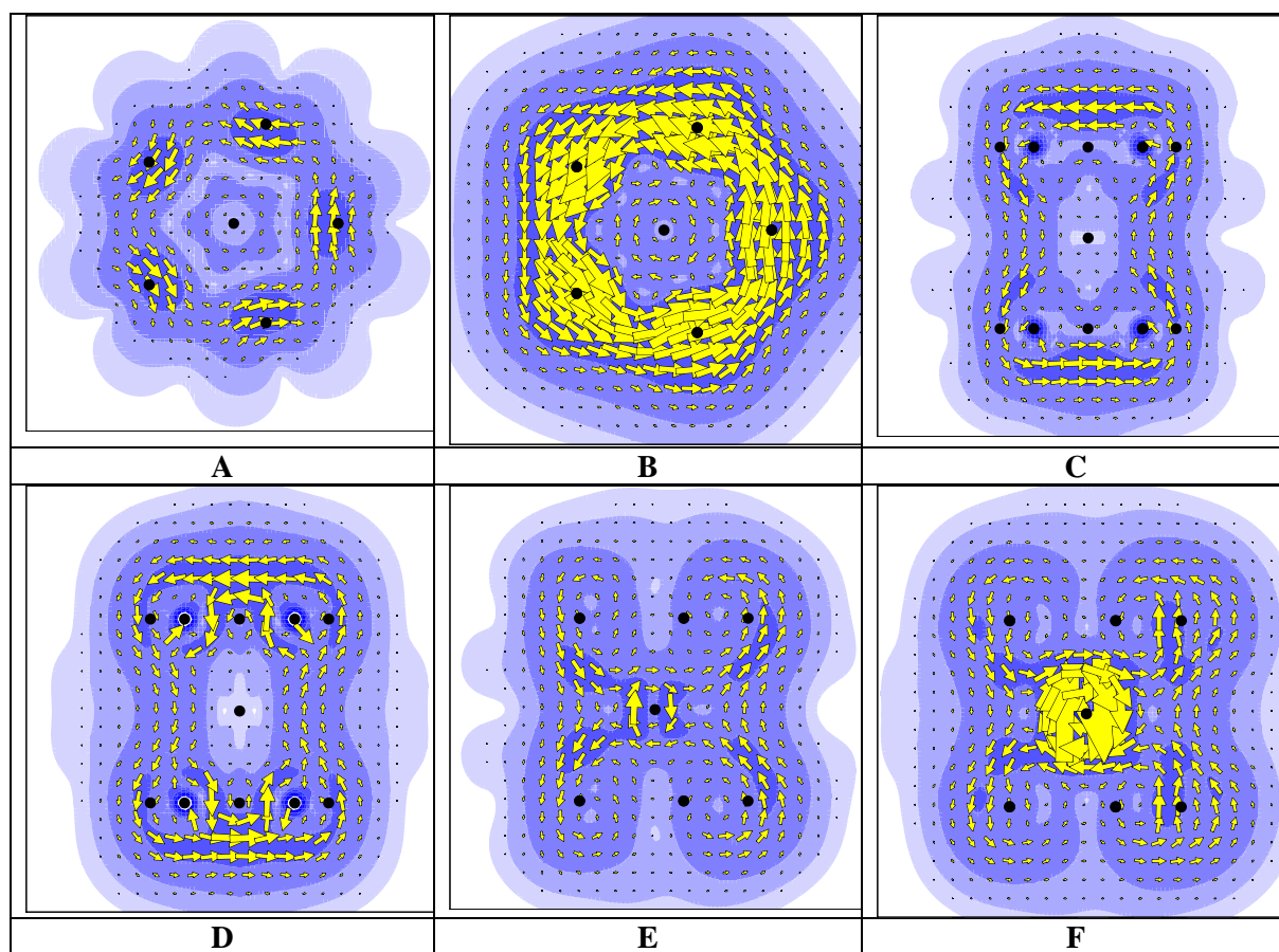
Ring currents of [\text{Ti}(\text{P}_5)_2]^{2-} (A) plane A \pi -orbital contribution, (B) plane A total orbital contribution, (C) plane B \pi -orbital contribution, (D) plane B total orbital contribution, (E) plane C \pi -orbital contribution, (F) plane C total orbital contribution.
