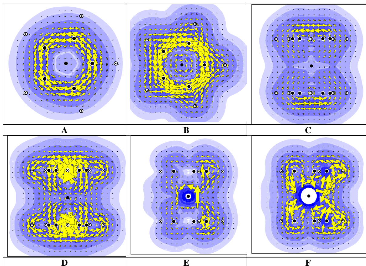
Ring currents of ferrocene (A) plane A \pi -orbital contribution, (B) plane A total orbital contribution, (C) plane B \pi -orbital contribution, (D) plane B total orbital contribution, (E) plane C \pi -orbital contribution, (F) plane C total orbital contribution.
