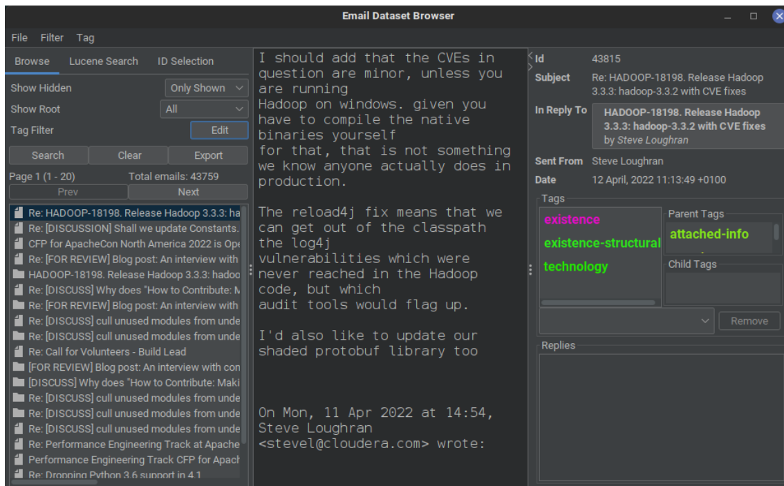
Figure 3: A screenshot of the email dataset browser app's main user interface, showing an email that has some tags.
