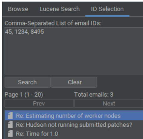
Figure 8: The view for searching the dataset using specific email ids.
