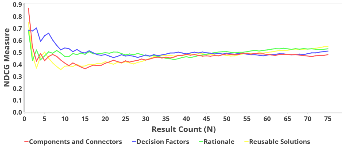
Figure 20: NDCG metric with thread relevance computed using all architectural design decision tags, for all queries.
