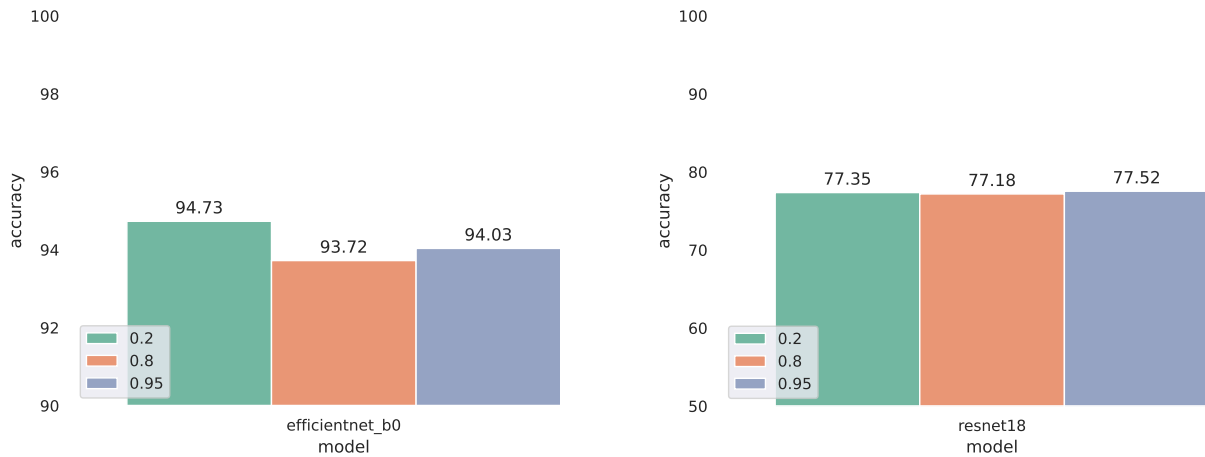
(a) EfficientNetB0 [70] trained with Proxy Attention on the Stanford Dogs dataset [63] (b) Resnet18 [27] trained with Proxy Attention on the Tsinghua Dogs Dataset [66]
