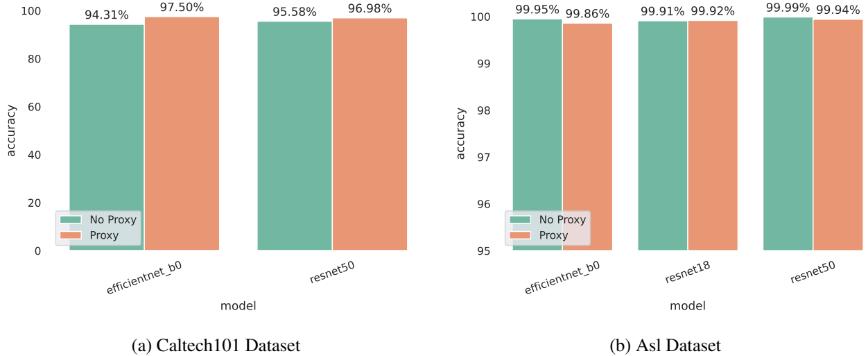
Figure 4.3: Comparing Accuracies of models trained with and without Proxy Attention on the Caltech101 and Asl datasets
