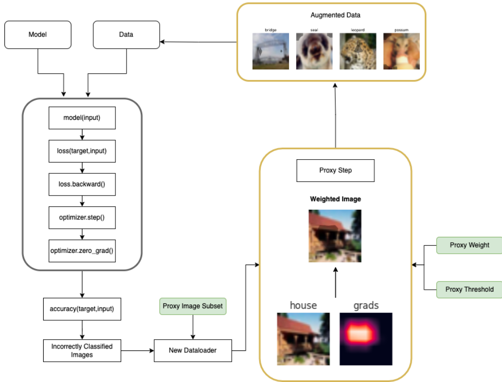
Figure 3.1: Proxy Attention Visualized
