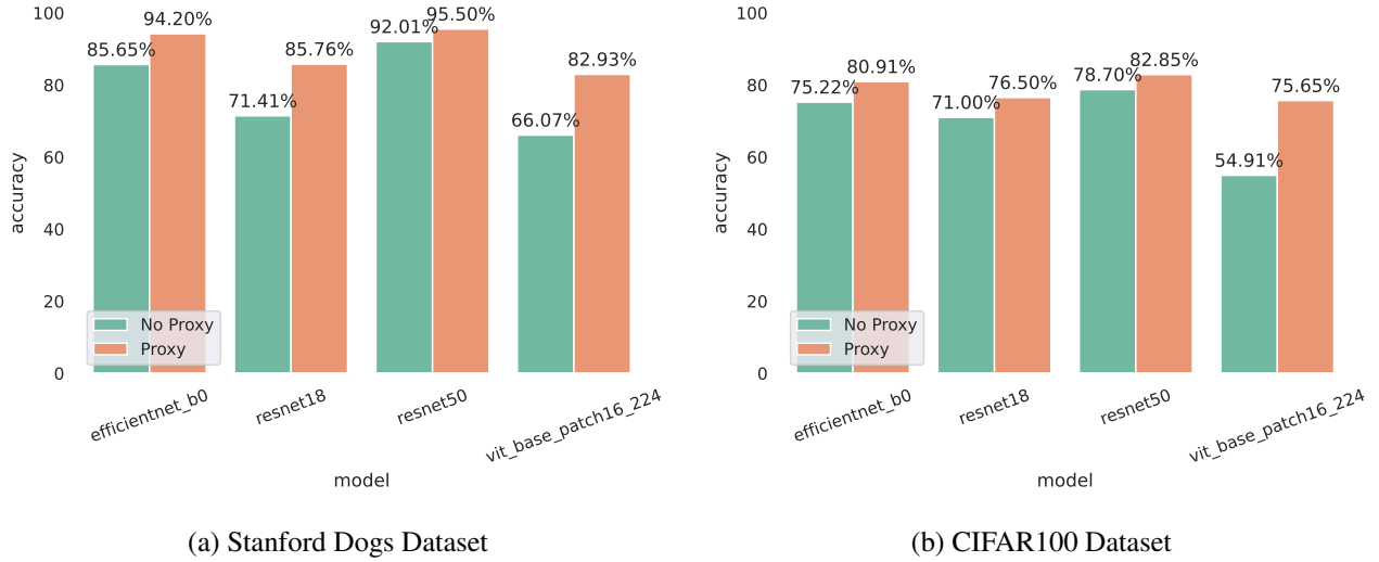
Figure 4.2: Comparing Accuracies of models trained with and without Proxy Attention on the Stanford Dogs and CIFAR100 datasets
