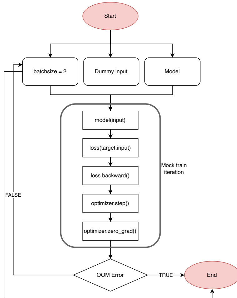
Figure 7.5: Diagrammatic representation of the Batch Size Finder Algorithm
