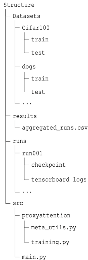
Figure 3.4: Code Directory Structure
