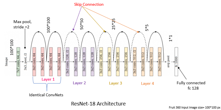
Figure 3.14: ResNet18 architecture
