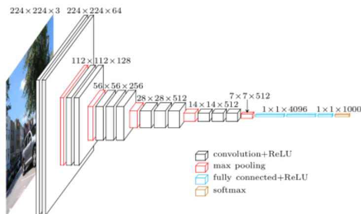
Figure 3.13: VGG16 architecture
