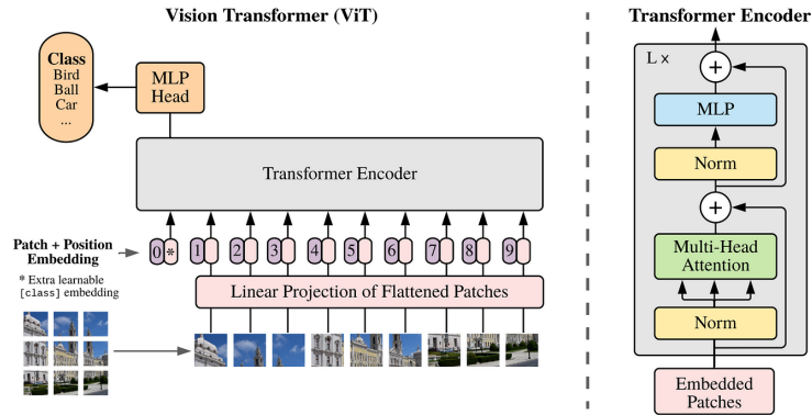
Figure 3.16: ViT Base Patch 16 \times 224 architecture
