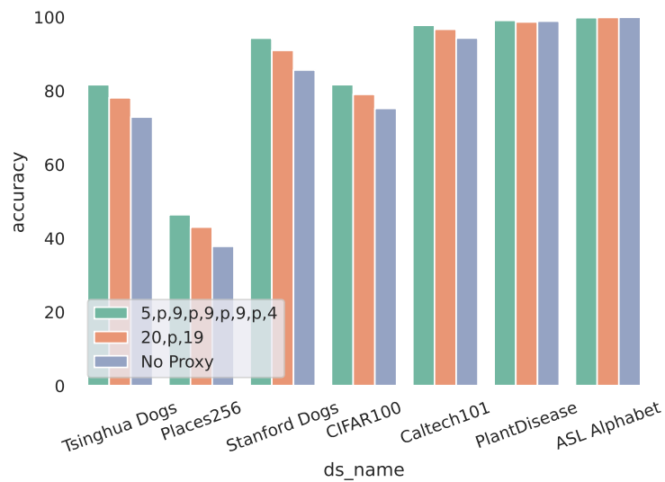
Figure 4.5: Comparing Accuracies of models trained with and without Proxy Attention on the ResNet50 [27] architecture for different step schedules
