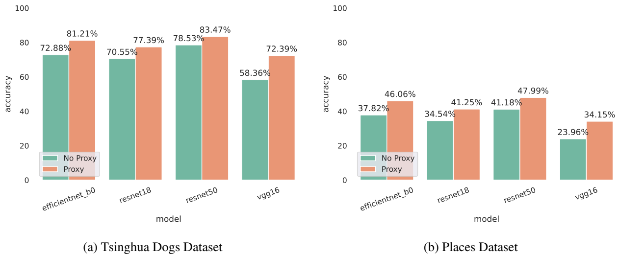
Figure 4.1: Comparing Accuracies of Models trained with and without Proxy Attention on the Tsinghua Dogs and Places datasets
