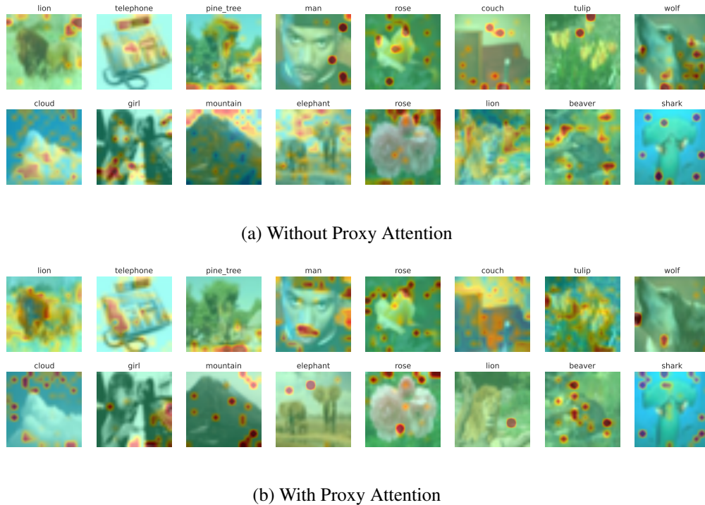
Figure 4.11: Comparison of attention maps generated by vit_base_patch16_224 trained with and without Proxy Attention on the CIFAR100 dataset
