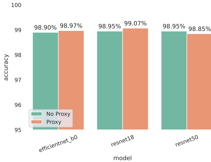
Figure 4.4: Comparing Accuracies of models trained with and without Proxy Attention on the Plant Disease dataset
