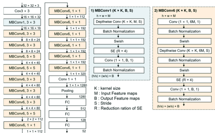
Figure 3.15: EfficientNetB0 architecture
