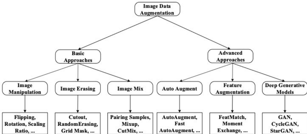
Figure 2.1: Taxonomy of Data Augmentation [29]
